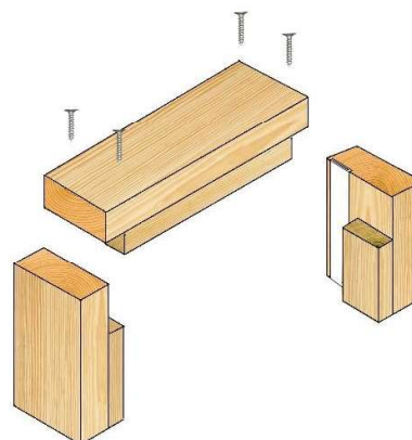
Butt Joint
